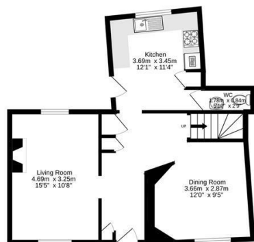
Ground Floor 51.6 sq.m. (556 sq.ft.) approx.
